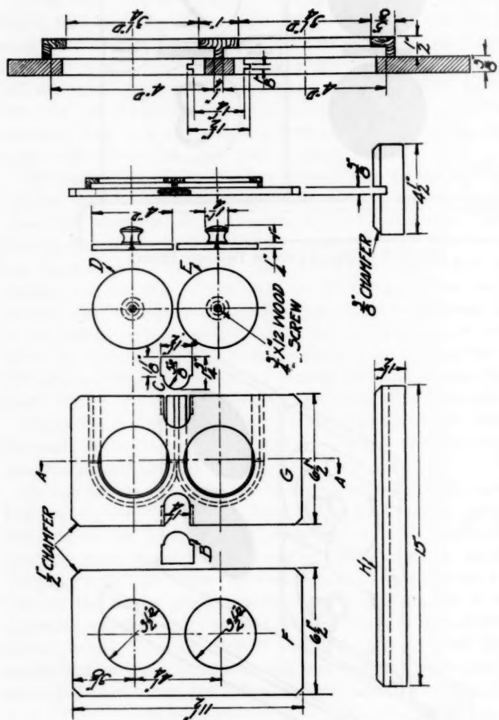
FIGURE III—DETAILED ORTHOGRAPHIC VIEW OF FRACTION DIVIDER, WITH DIMENSIONS OF ALL PARTS GIVEN IN INCHES
